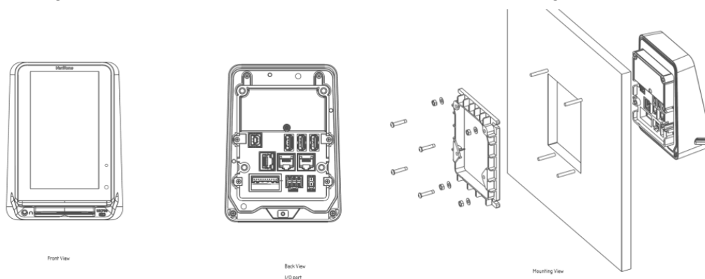
Figure 6 Mounting the UX700
