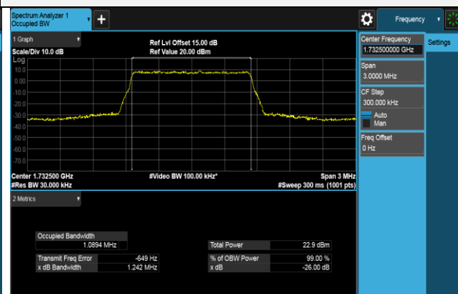
26 dB Bandwidth
