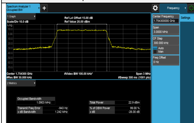
Occupied bandwidth
