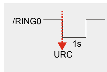
Figure 26: URC transmission
