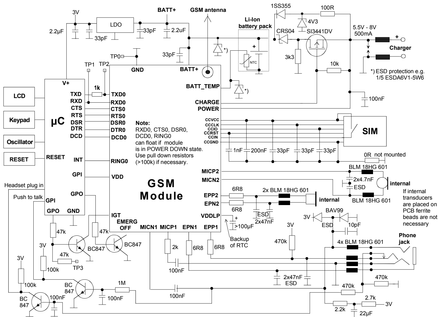
Figure 47: Schematic diagram of MC55/56 sample application
