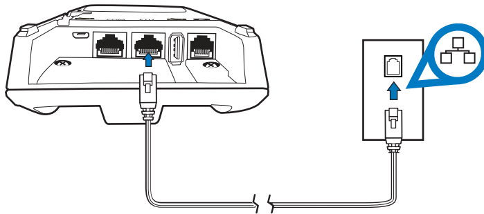
Figure 16 Ethernet Connection
