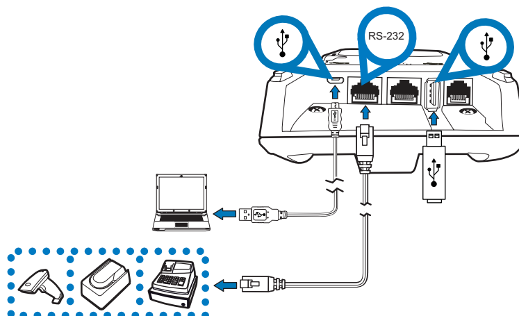
Figure 18 Connecting Peripheral Devices
