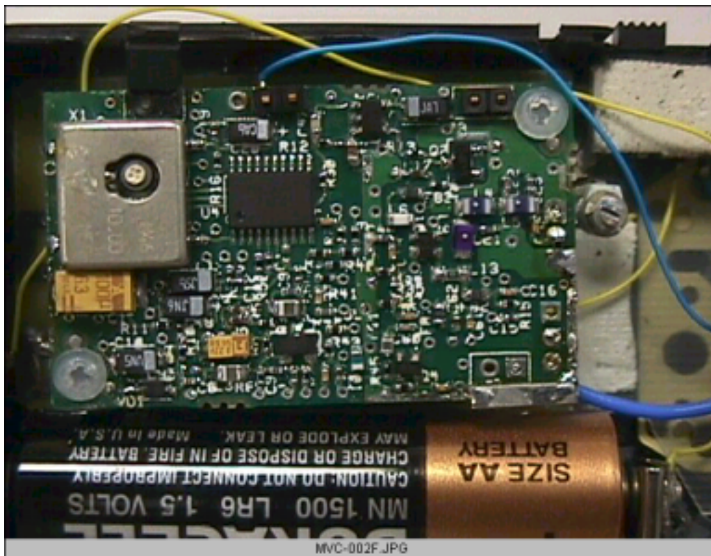
AID2 - PCB Component Side of FM Transmitter
