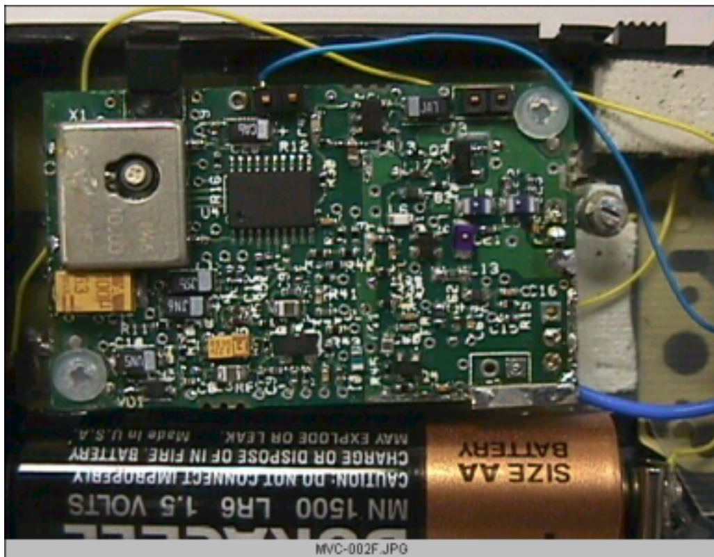
AID - PCB Component Side of FM Transmitter
