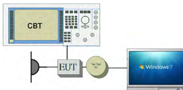
Fig.2-2 Conducted Emission (Antenna Port) Configuration
