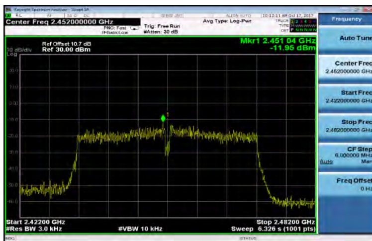
802.11n_40 CH-High
