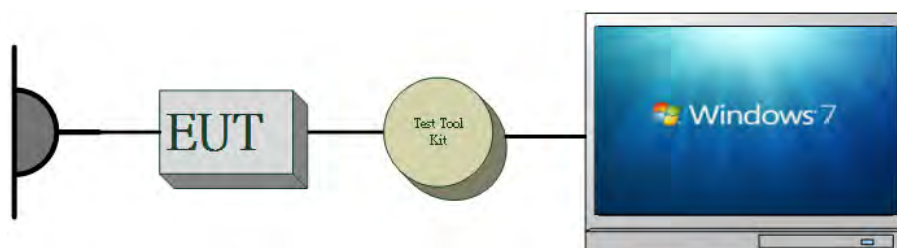
Fig. 2-2 AC Power Line Conducted Emission Configuration
