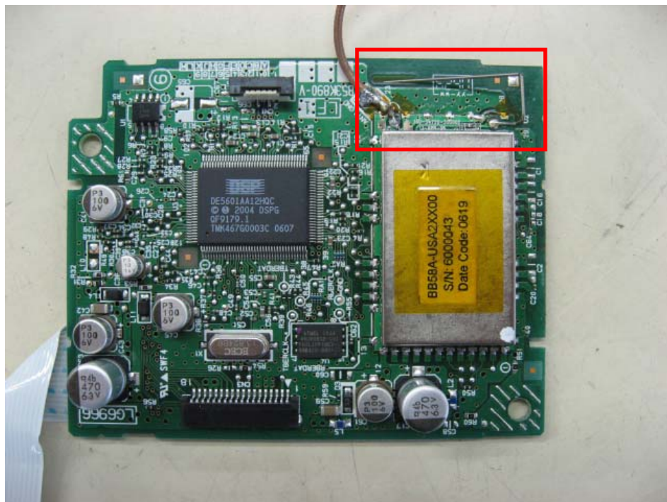
Wire antenna
