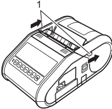
1 Peeler latch
