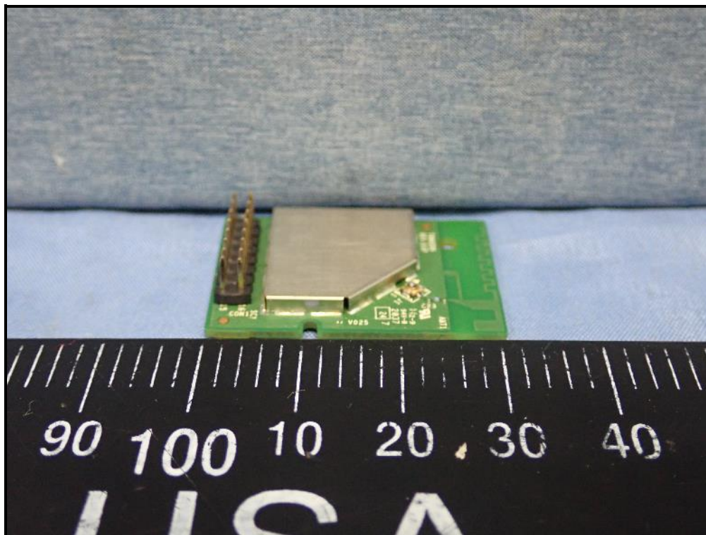
Type 1: 16 pin
