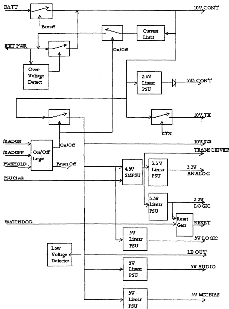
Figure 2-3 Guardian Power Supply
