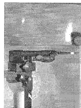
Body-worn SAR Test Setup with 1.5cm separation distance
