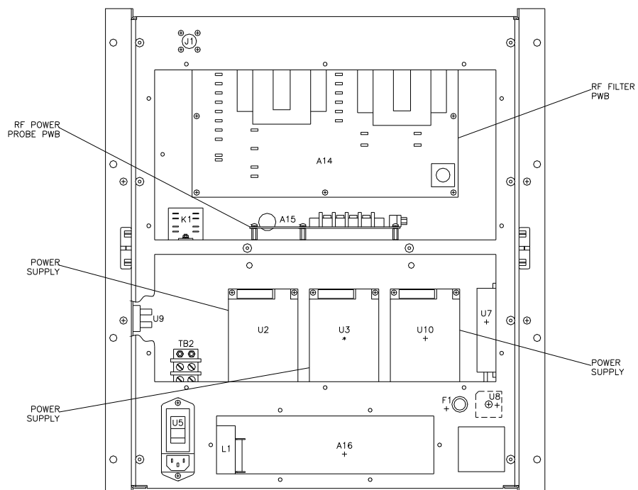
Figure 4-1 Exciter Panel and Rear View
