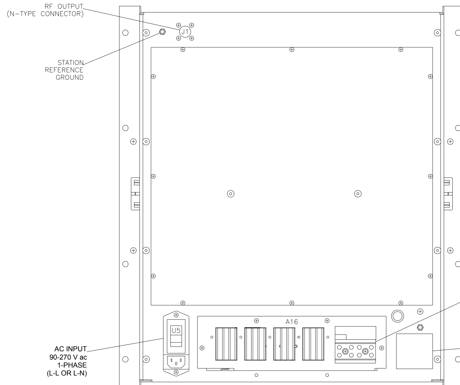
BACK OF TRANSMITTER
