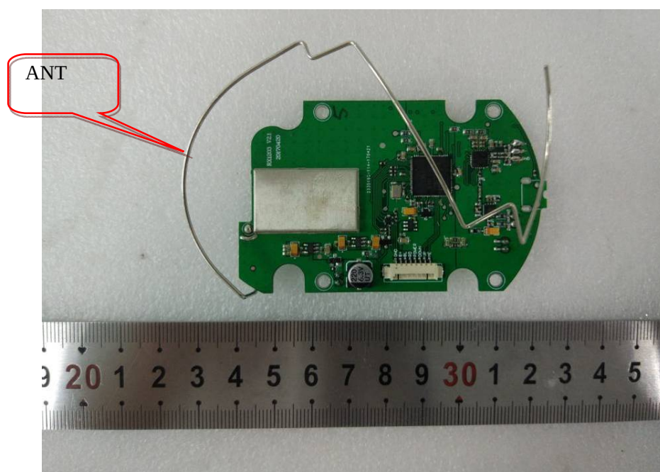
EUT – Main Board 1Top View
