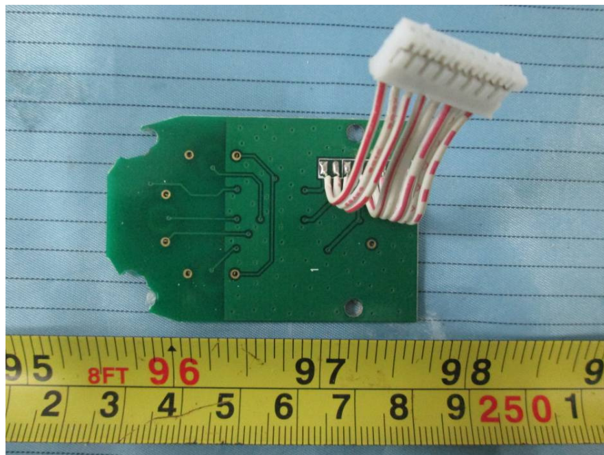
EUT –Button PCB Back View
