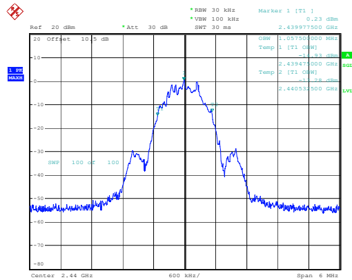
Middle Channel 1.058MHz
