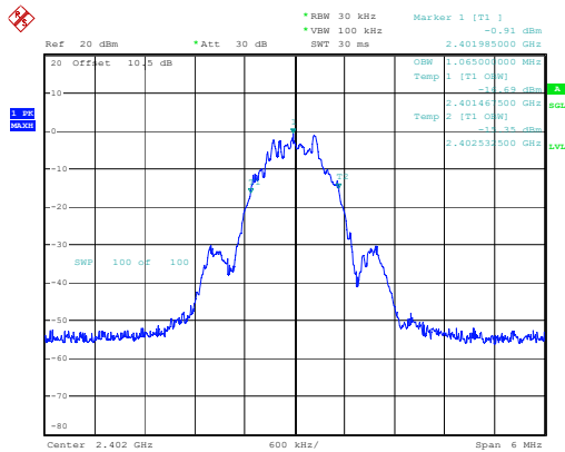
Low Channel 1.065MHz
