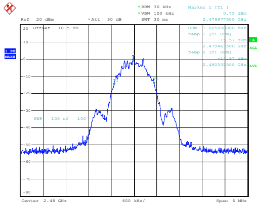
High Channel 1.065MHz
