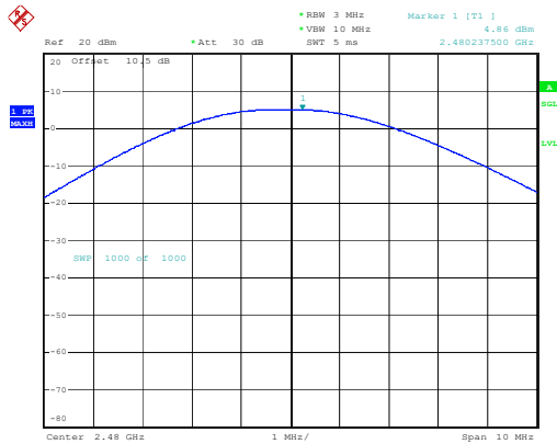
High Channel 4.86dBm
