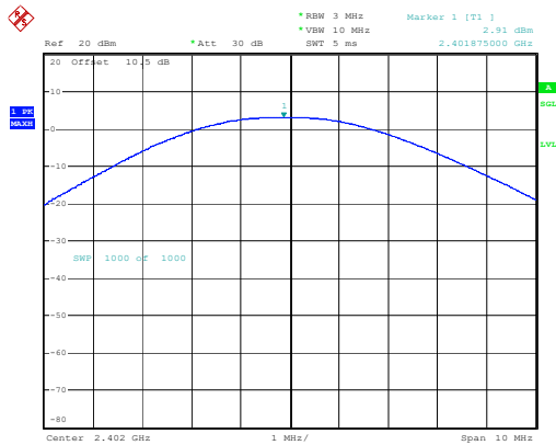
Low Channel 2.91dBm
