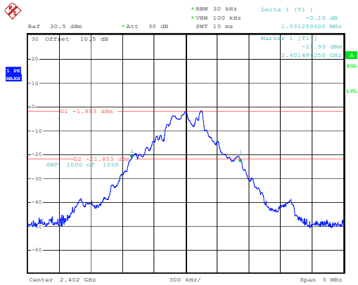
GFSK_Low 1.031MHz
