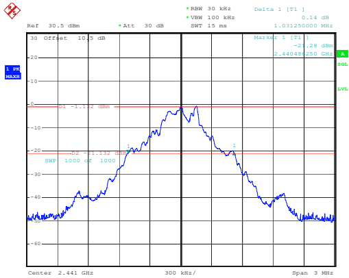
GFSK_Middle 1.031MHz
