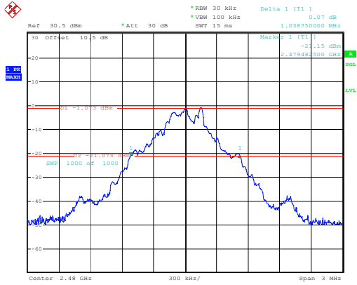
GFSK_High 1.039MHz
