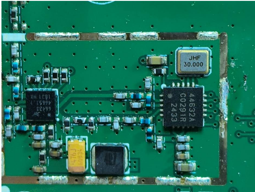
SRD Antenna
