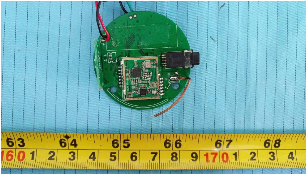
EUT – Main Board Bottom Cover off View
