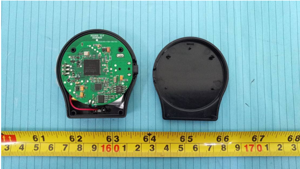
EUT – Cover off View 1
