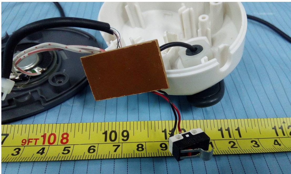
EUT (Headset 2) – Main Board Bottom View
