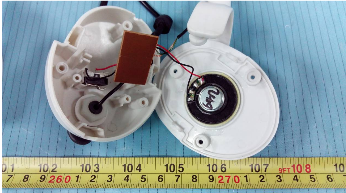
EUT (Headset 1) – Main Board Bottom View
