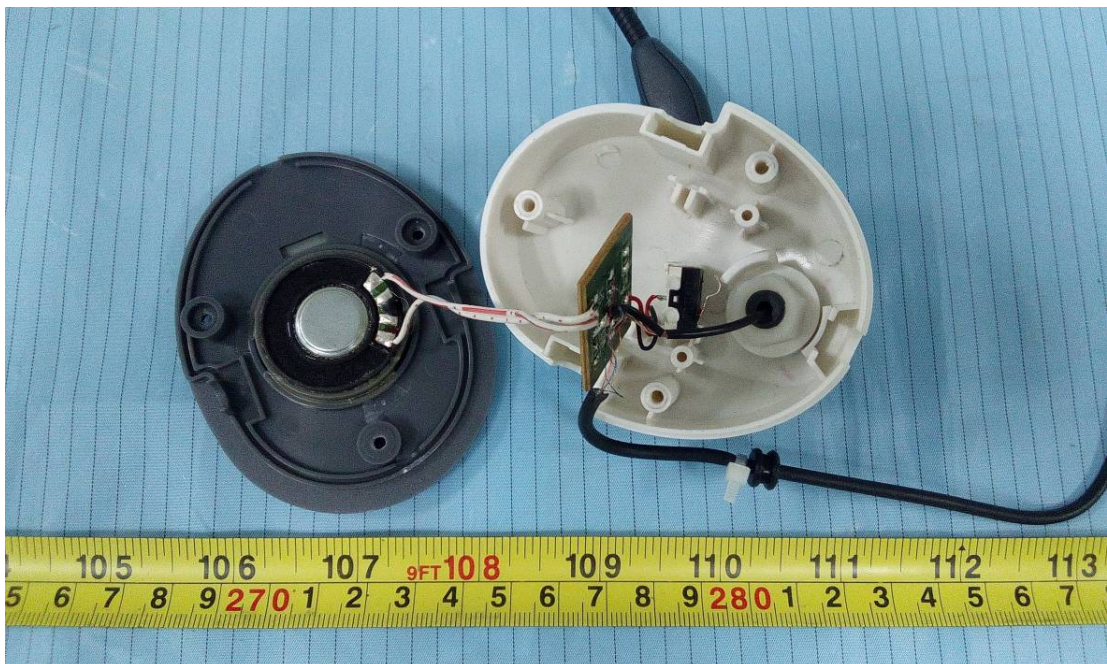
EUT (Headset 2) – Cover off View 3
