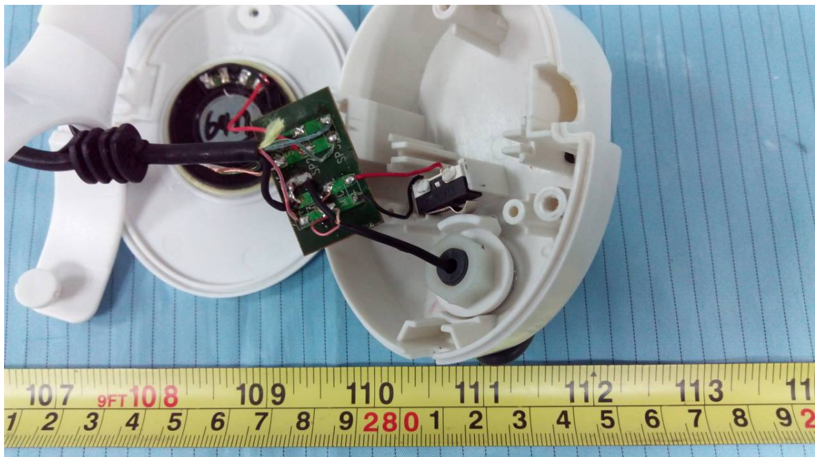
EUT (Headset 1) – Main Board Top View
