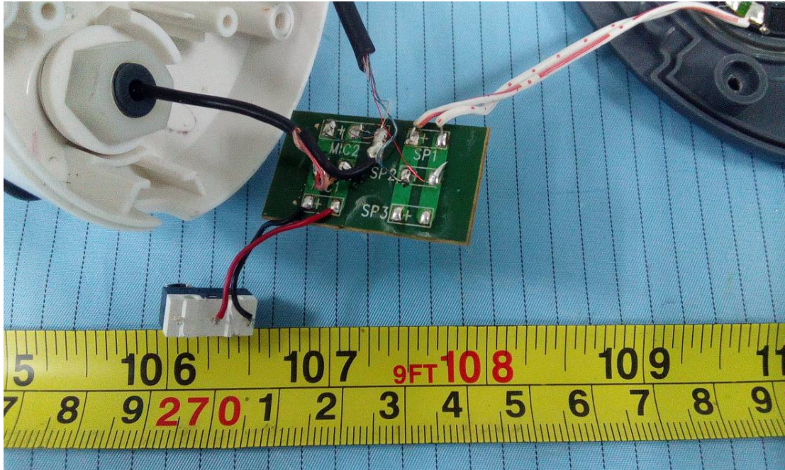
EUT (Headset 2) – Main Board Top View
