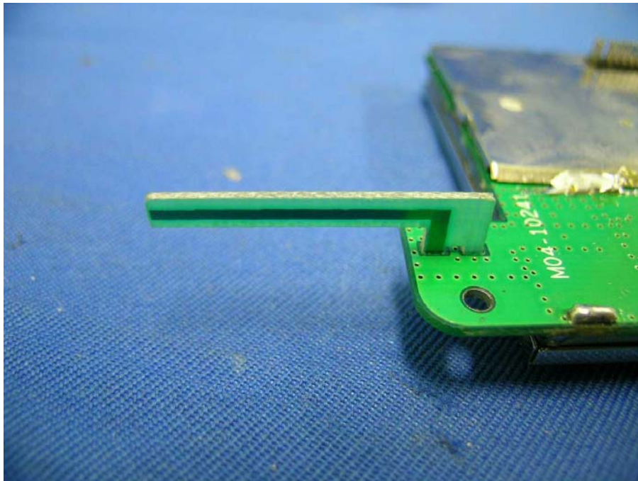
Master Unit TX Antenna PCB front side
