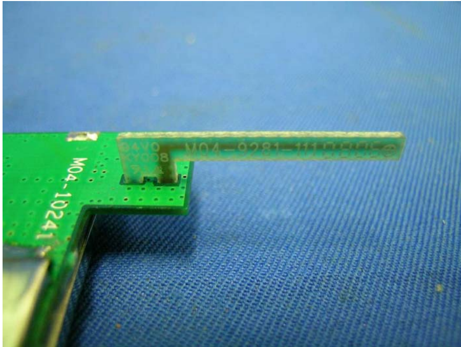
Remote Unit TX Antenna PCB rear side
