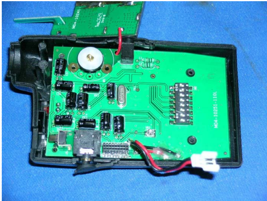
Master Unit Main PCB comp side
