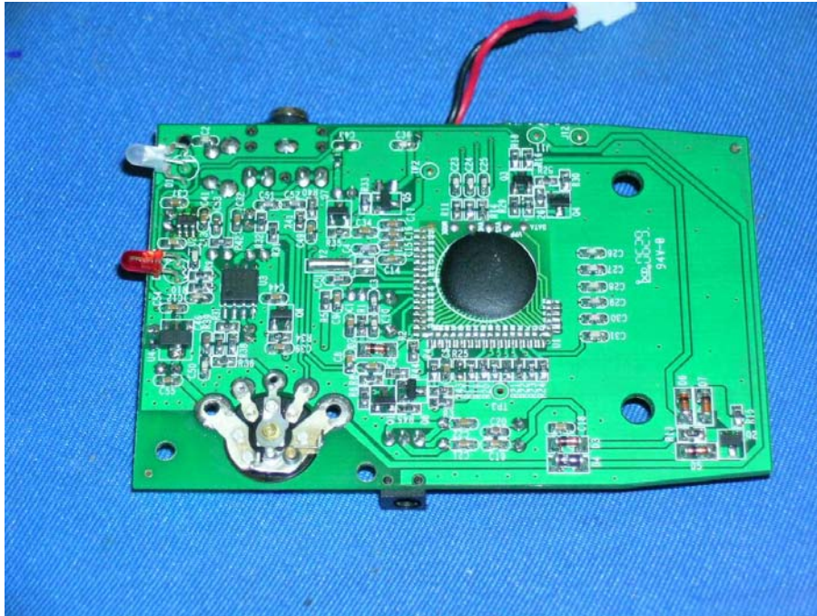
Master Unit Main PCB solder side
