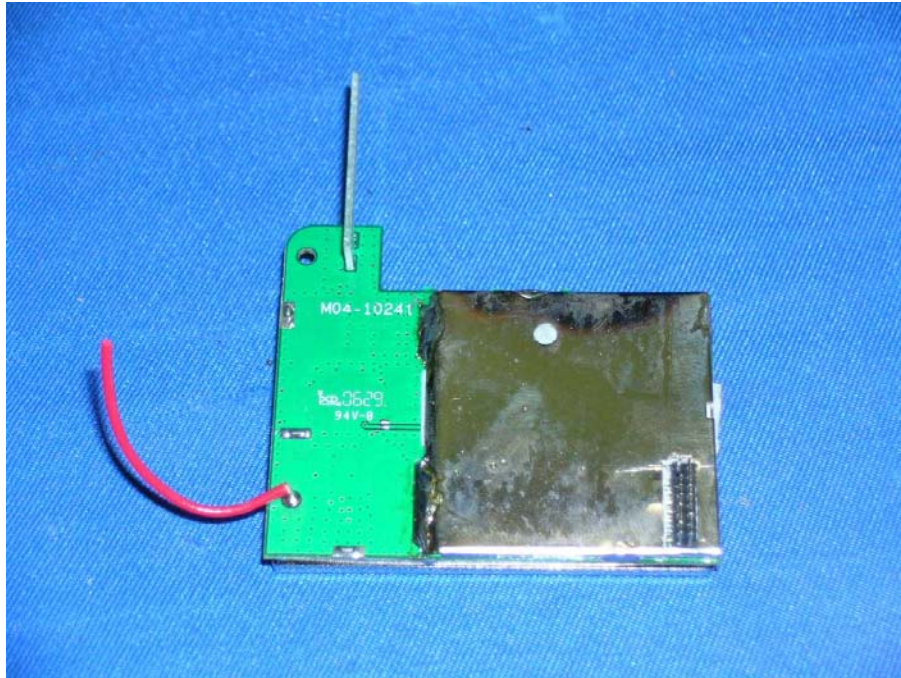
Remote Unit Oscillator PCB solder side (View 1)
