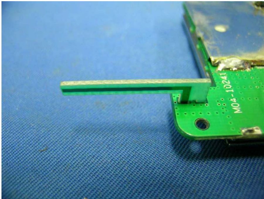
Remote Unit TX Antenna PCB front side
