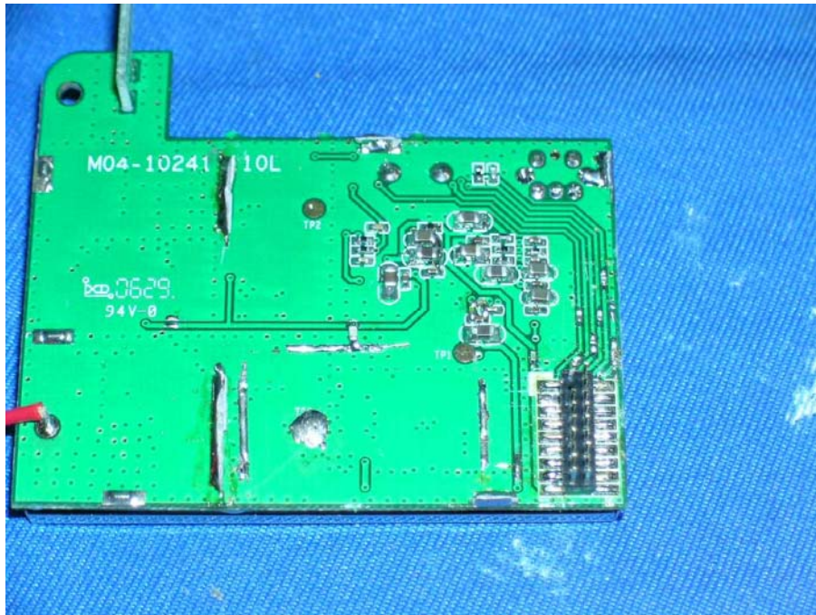
Remote Unit Oscillator PCB solder side (View 2)
