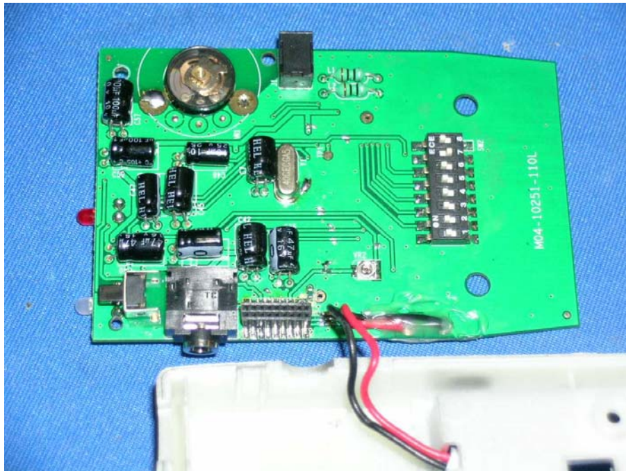
Remote Unit Main PCB comp side
