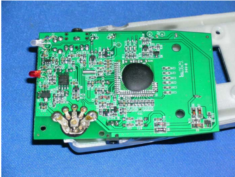
Remote Unit Main PCB solder side
