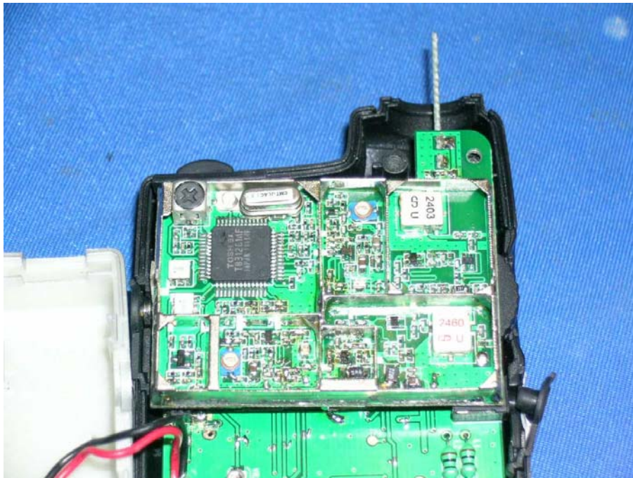
Remote Unit Oscillator PCB comp side
