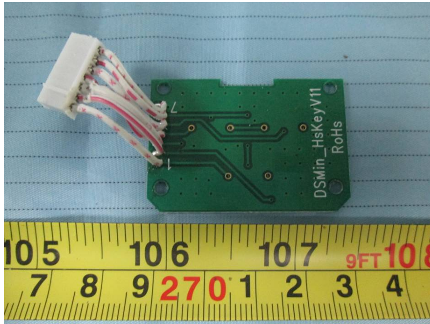
EUT – Control Panel Rear View
