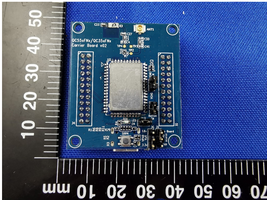
Ceramic Chip Antenna
