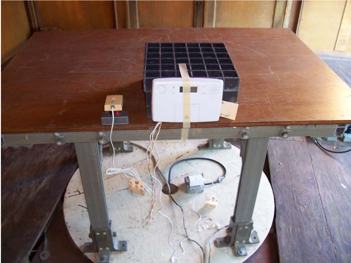
Radiated Emissions Y-Axis
