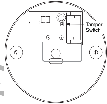
Figure 1. Tamper Switch Location
