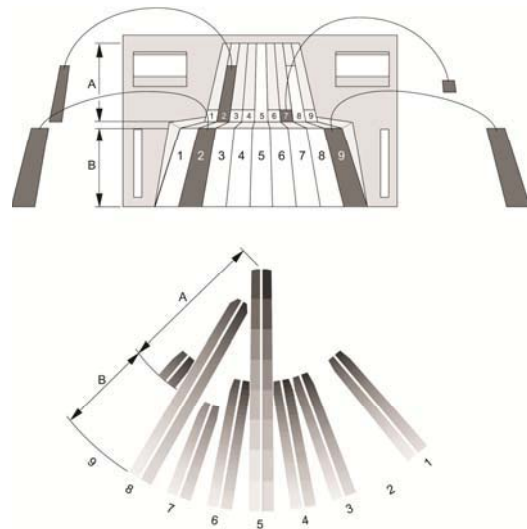
Figure 8: Installing Self-Adhesive Masks
