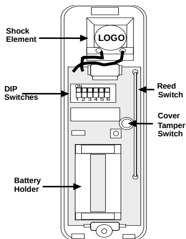
Figure 1. Shock Sensor Main Components
