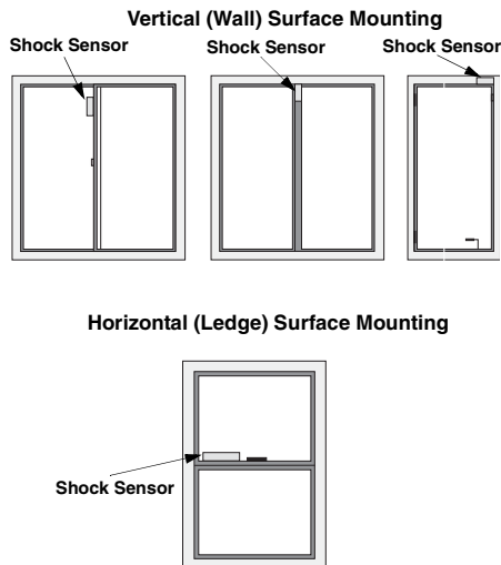
Figure 1. Mounting Options for Door/Window Sensor
