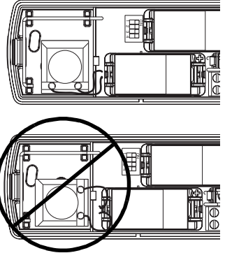
Figure 5. Positioning Shock Elements for Horizontal Surface Mounting
