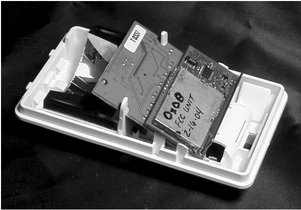
Figure 1: Picture of DUT, showing transmitter board plugged on the motherboard.
