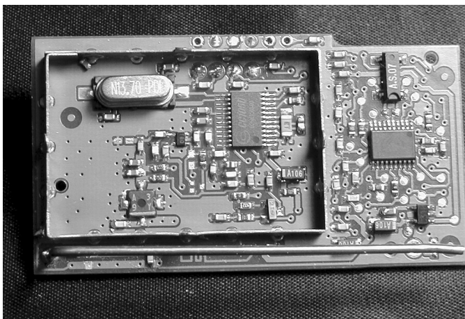
Figure 3: Picture of board with shield off.
