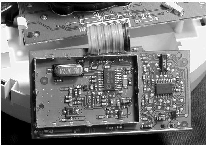
Figure 2: Picture of board with shield off.
