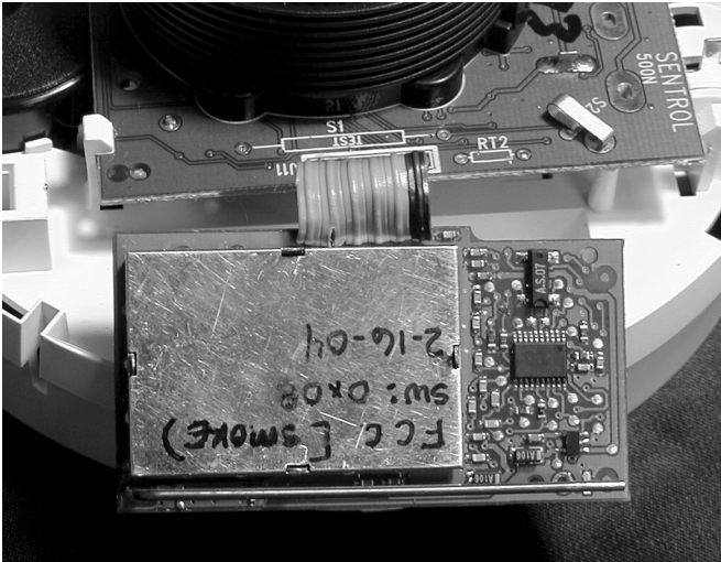
Figure 1: Picture of board with shield on.
