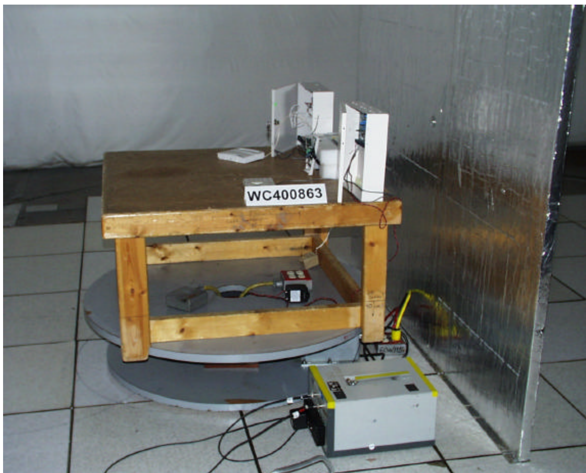
Figure 3: Picture of test setup for conducted emissions testing.
