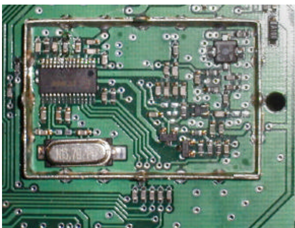
Figure 4: Picture of circuitry under RF shield.
