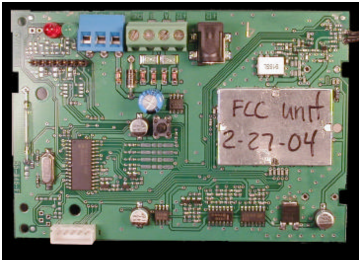
Figure 2: Close-up picture of DUT.
