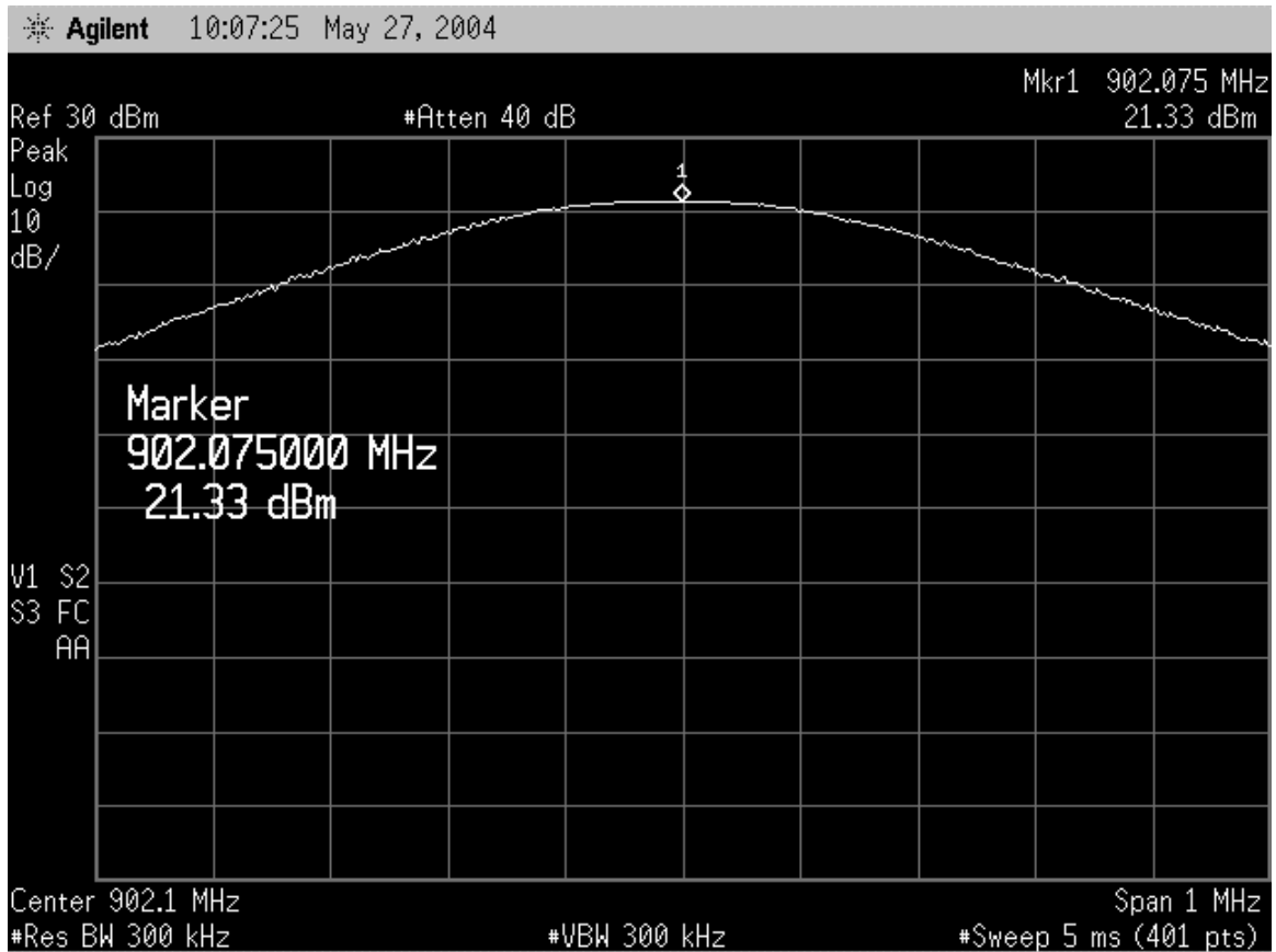
Figure 1: Peak conducted output power, low channel.
