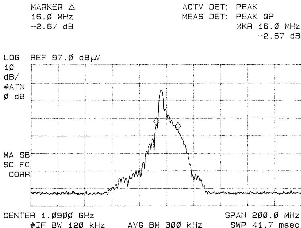
Figure 3: Occupied BandWidth.
