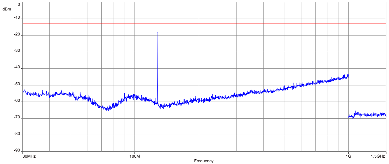
Plot 2: 127.500, 8.33 kHz channel bandwidth
