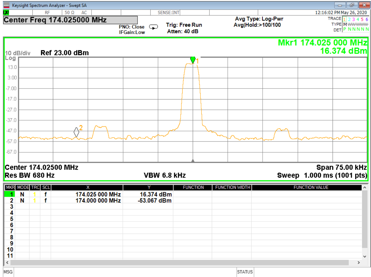
Figure 22 - Channel Frequency, 174.025
