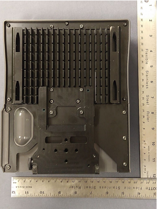
AP-1000 Back with No Mounting Plate
