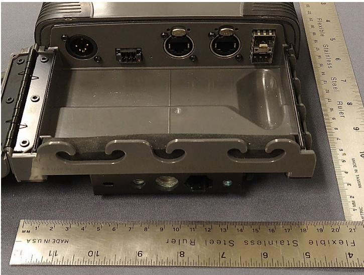
AP-1000 Bottom with Door Open
