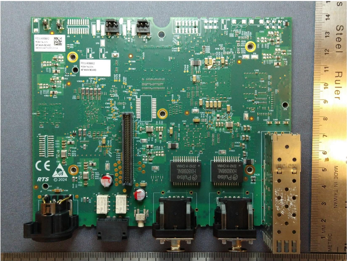
AP-1000 Main PCBA - Front
