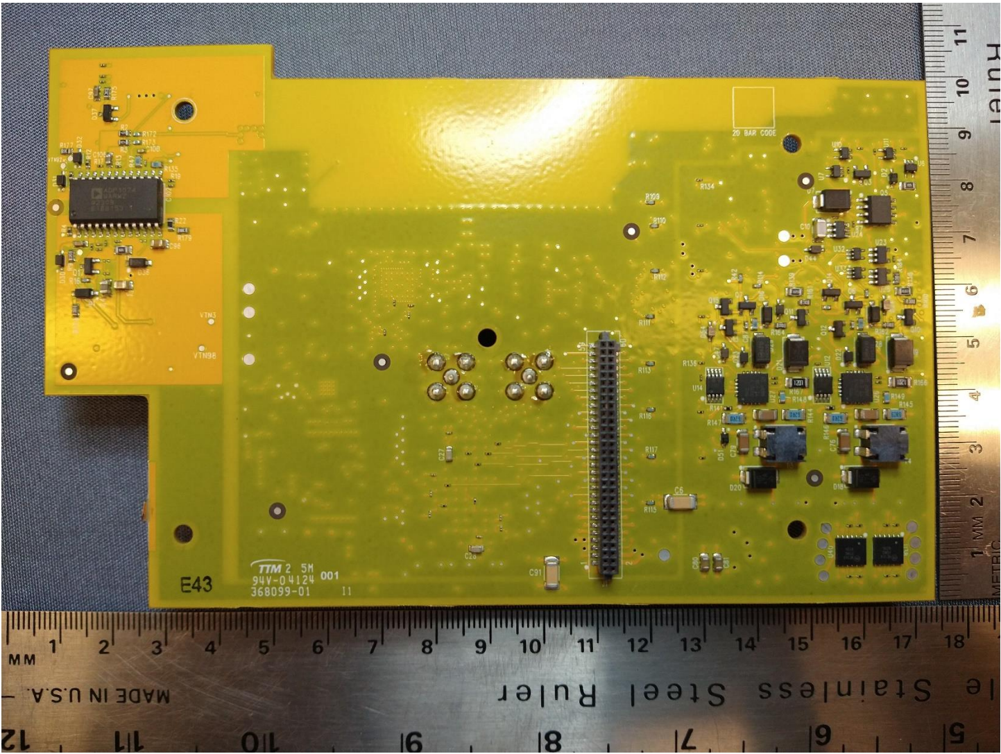
AP-1000 RF PCBA -Back
