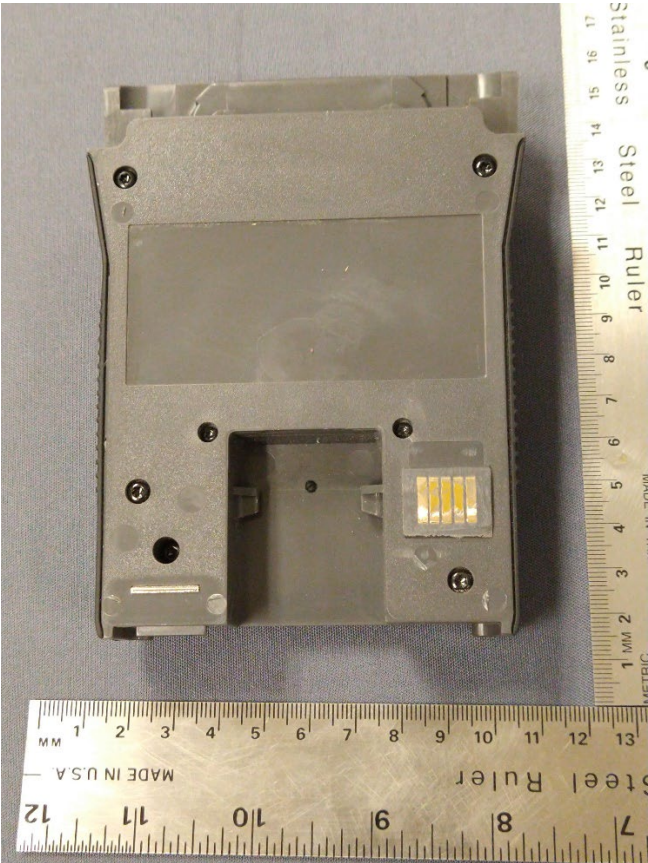
Battery Pack Front
