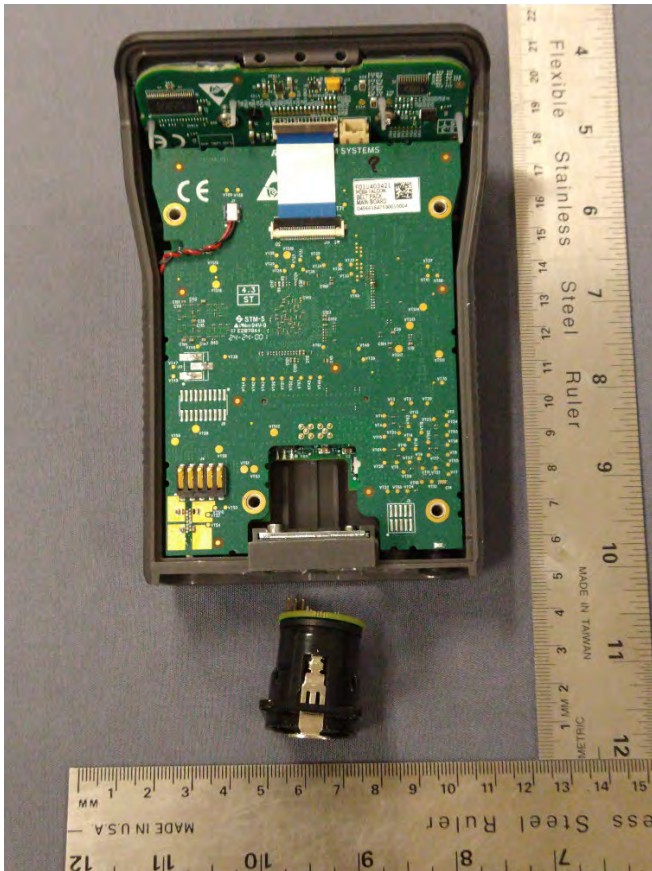
TR-1000 Main PCBA – Front
