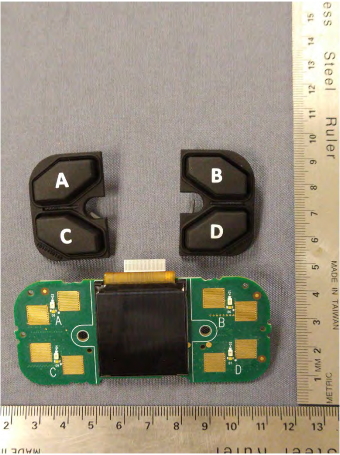
TR-1000 Top PCBA - Front
