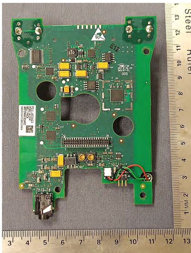
TR-1000 Antenna PCBA - Back
