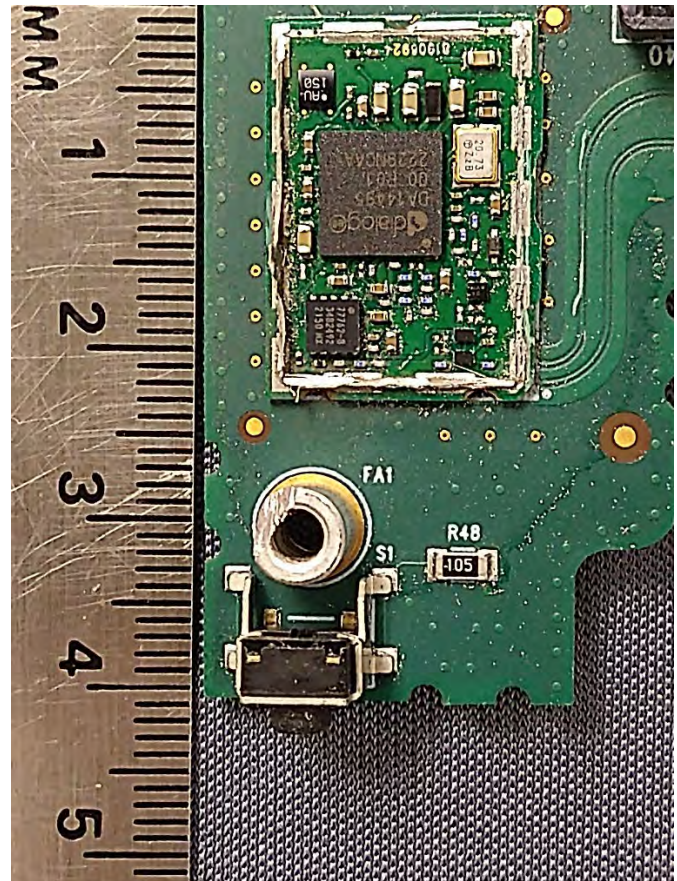
TR-1000 Main PCBA – RTX-1090 No Shield
