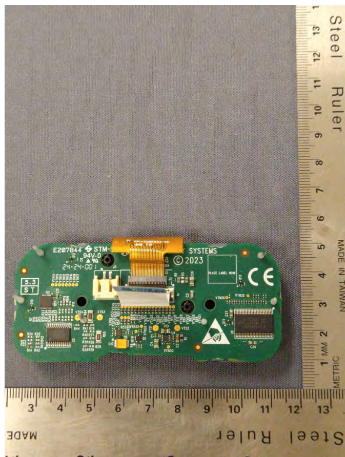
TR-1000 Top PCBA - Back
