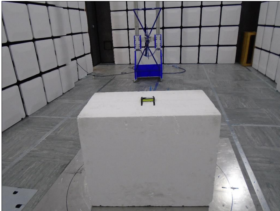
Figure 3 – Radiated Spurious Emissions - 30 MHz to 1 GHz, Orientation Z
