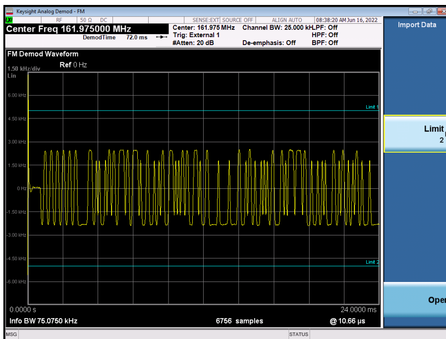
Figure 23- 161.975 MHz - PRBS
