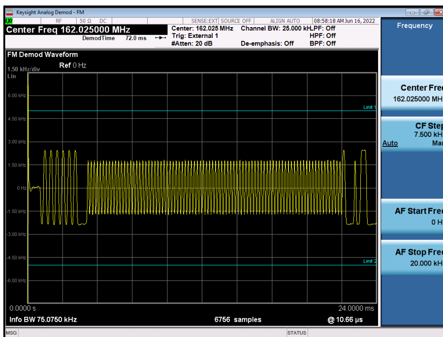
Figure 24 - 162.025 MHz - 01010101
