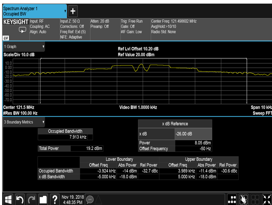
Figure 9 - 99% Occupied Bandwidth
