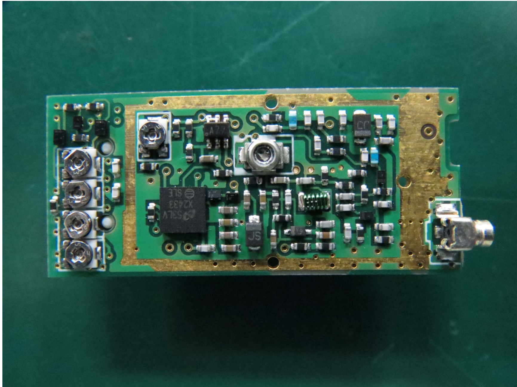
VC0-C14B Top (without Shield)
