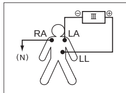
Lead III
