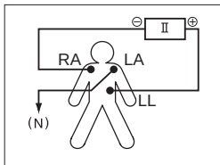
Lead II
