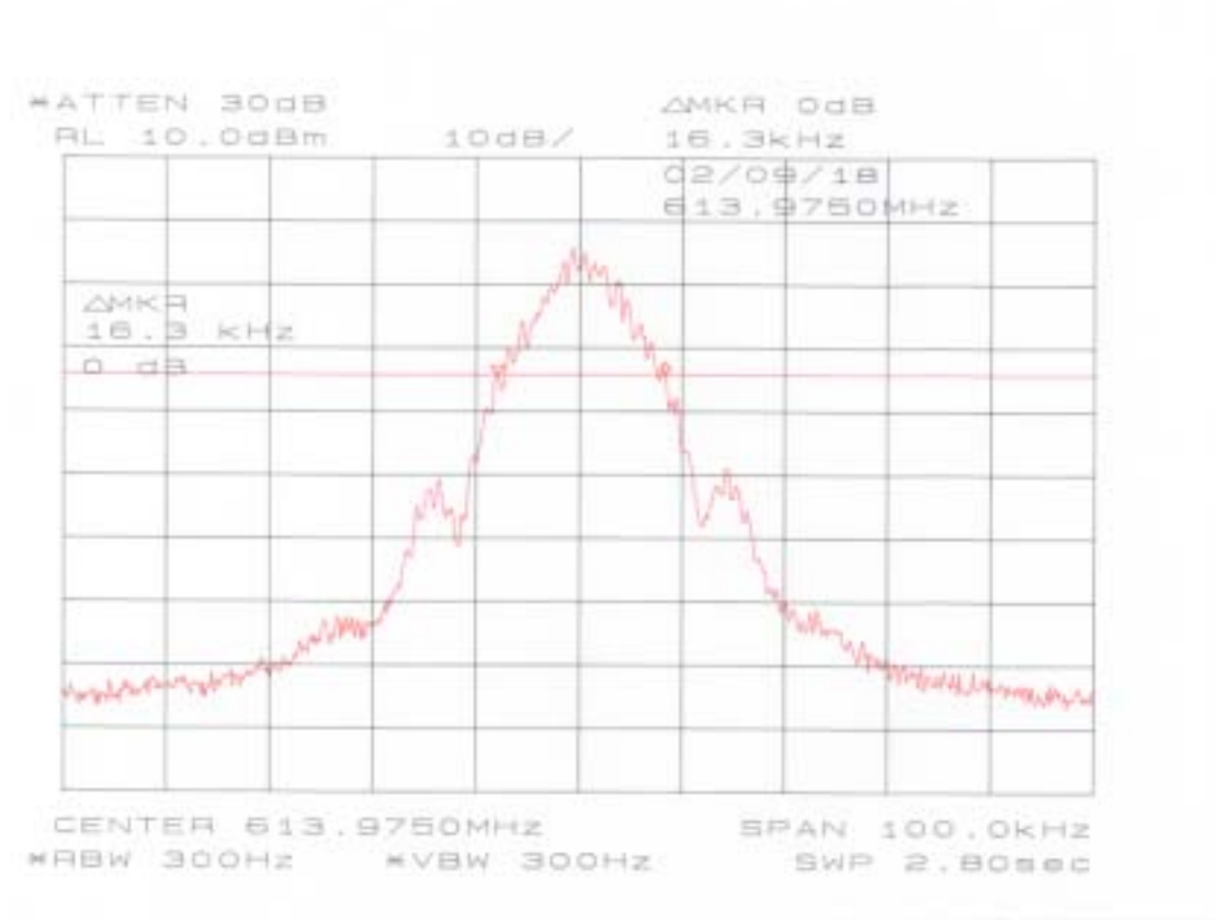
Chart of Channel (High : 613.9750 MHz)
