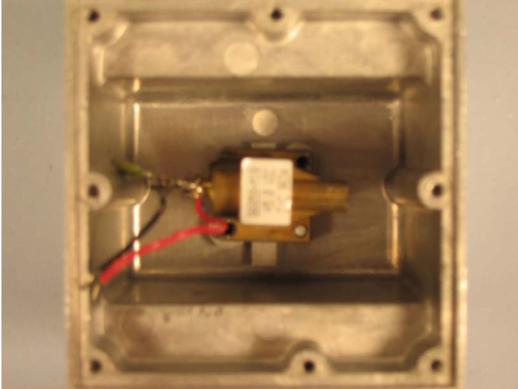
mn: 46783-1000, Transceiver in housing with wires
