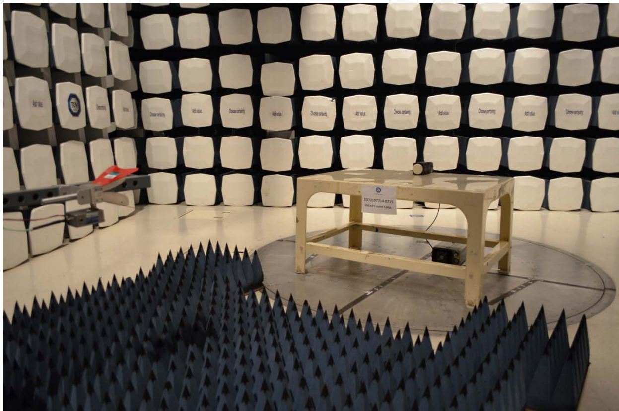
From 1 GHz to 18 GHz (Front)
