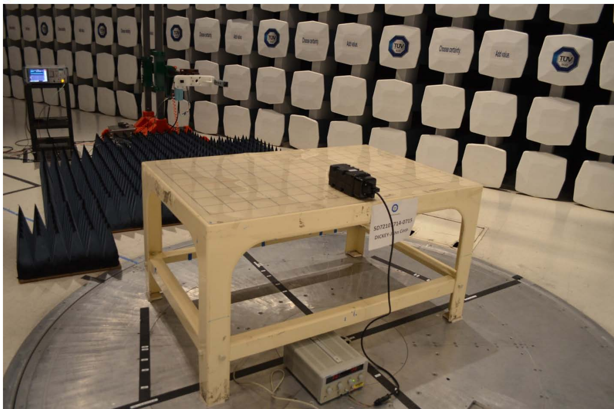
From 18 GHz to 26 GHz (Back)
