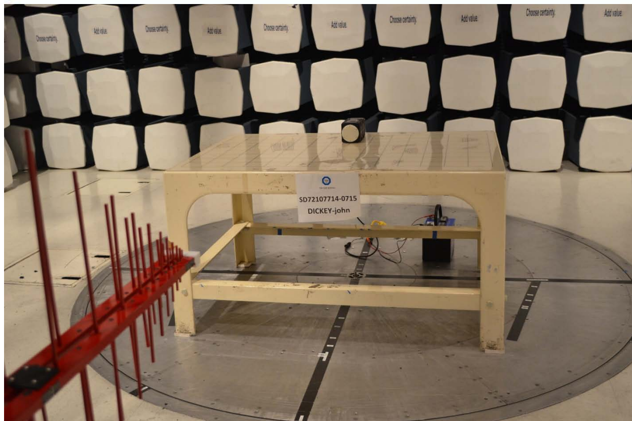
Below 1 GHz (Front)
