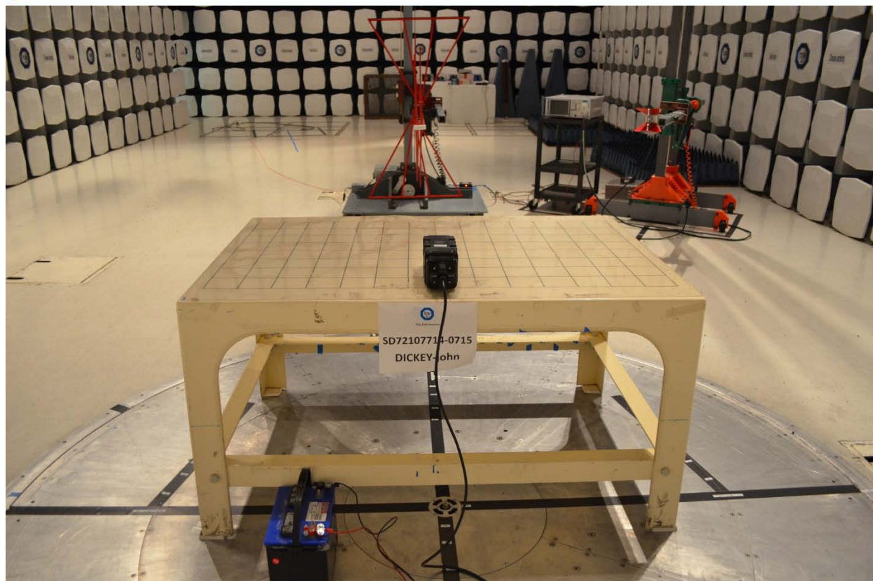
Below 1 GHz (Back)
